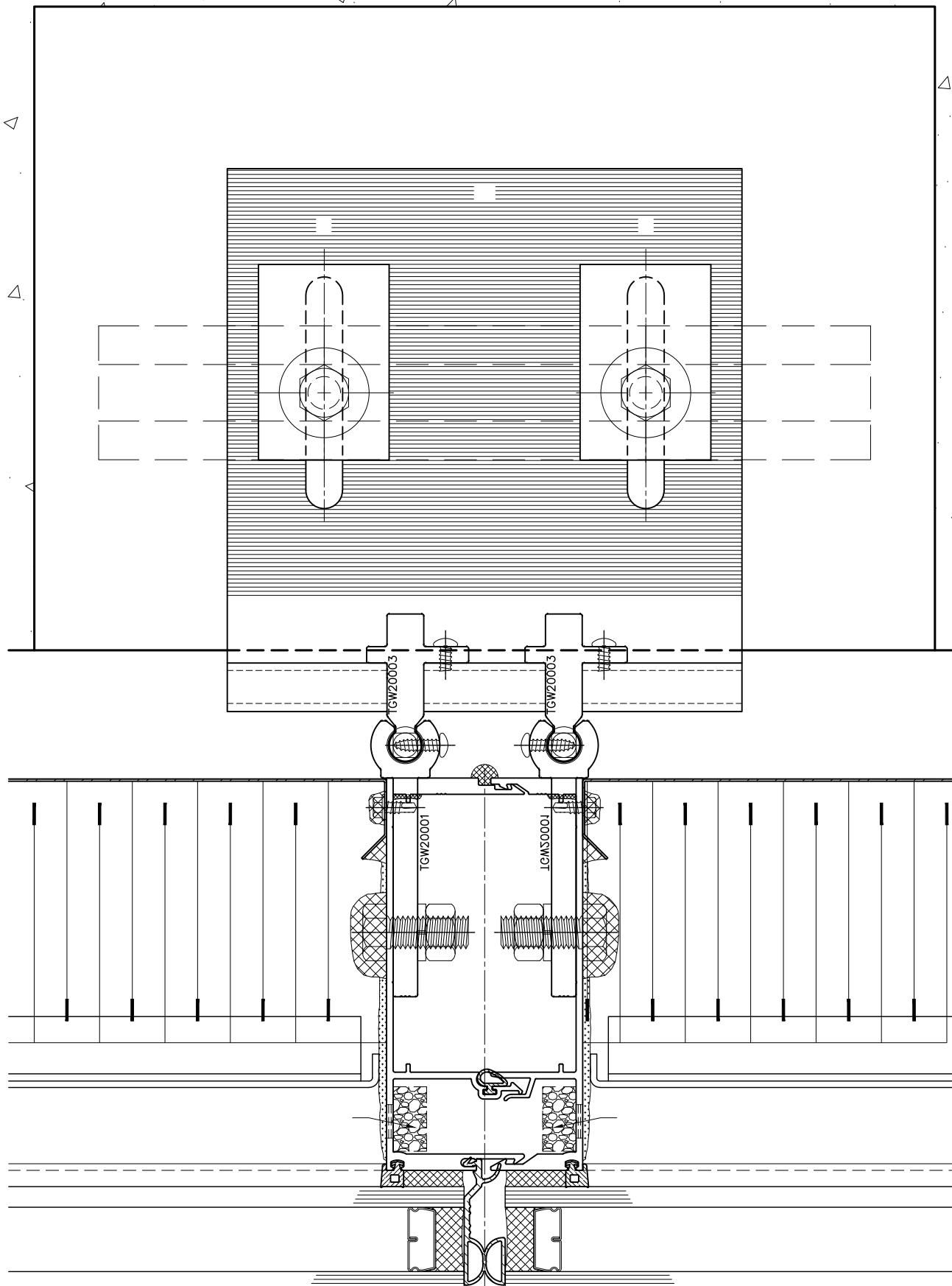
① TYPICAL PLAN DETAIL @ SLAB ANCHOR
